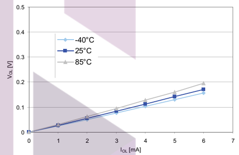
Figure 23. Typ. V_{OL} @ V_{DD} = 1.8 V (true open drain ports)
